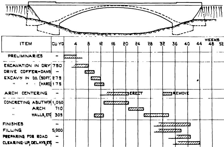
Fig. 267.—Estimating Contract Time.
